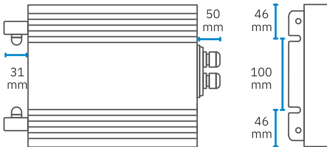
Protruding connectors
